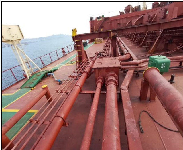
33. View of spring Btw 1-2 Pedestal Roller Guide.
