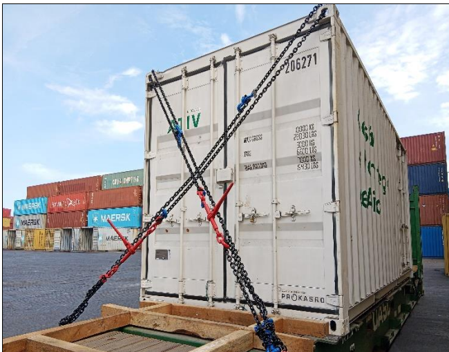
7. Use of chains for Lashing WLL 3,200 ton.
